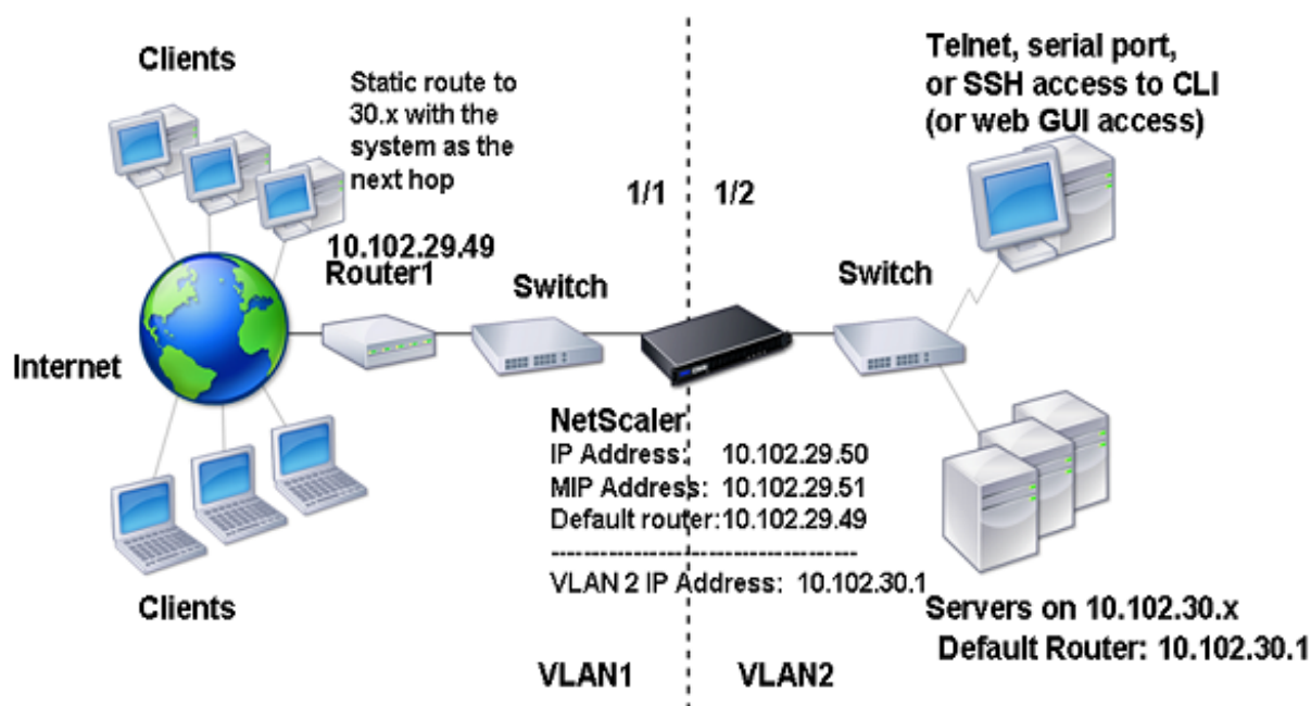
Figure 1. Multiple Subnets with VLANs - No Tagging
