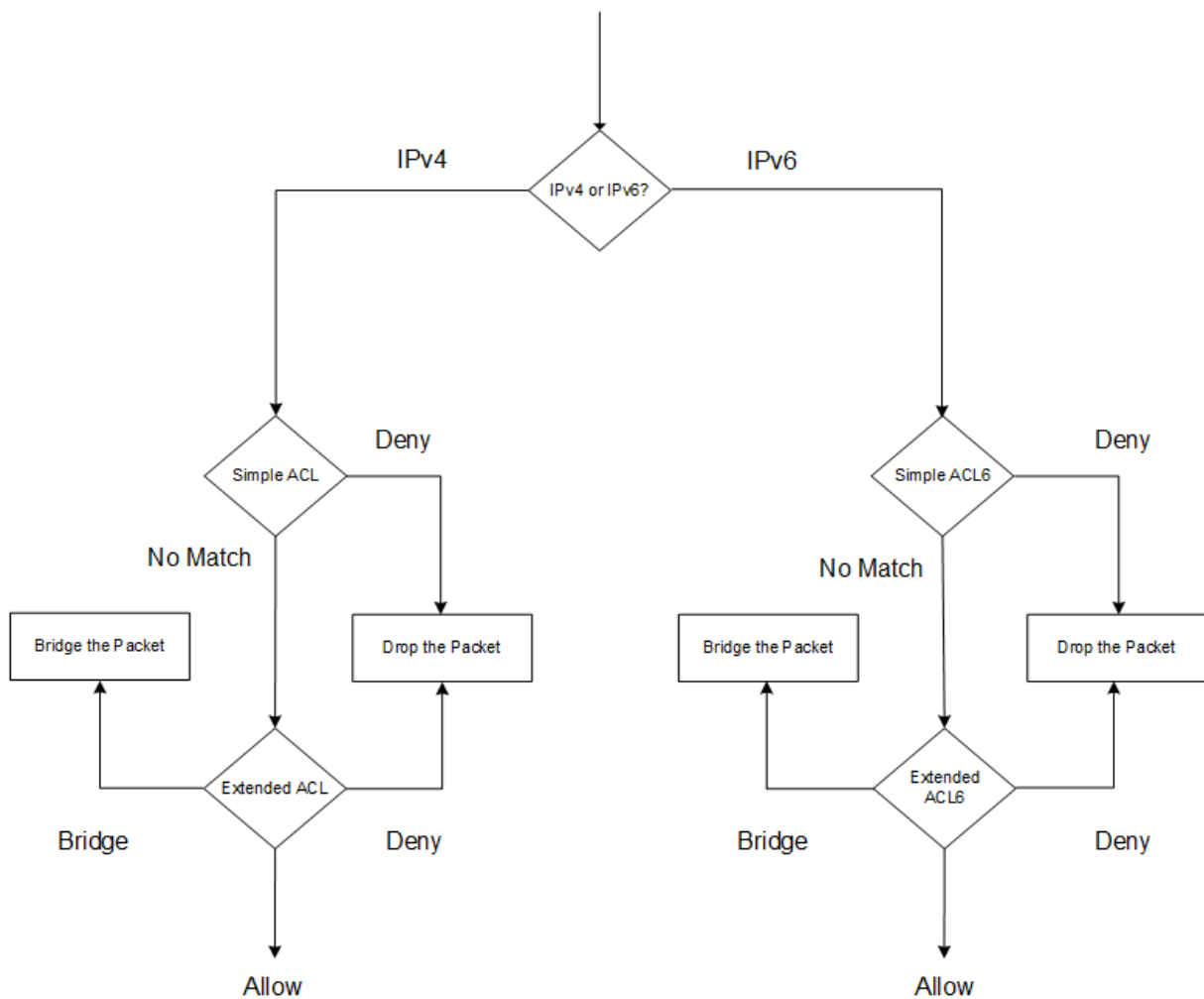
Figure 1. Simple and Extended ACLs Flow Sequence
