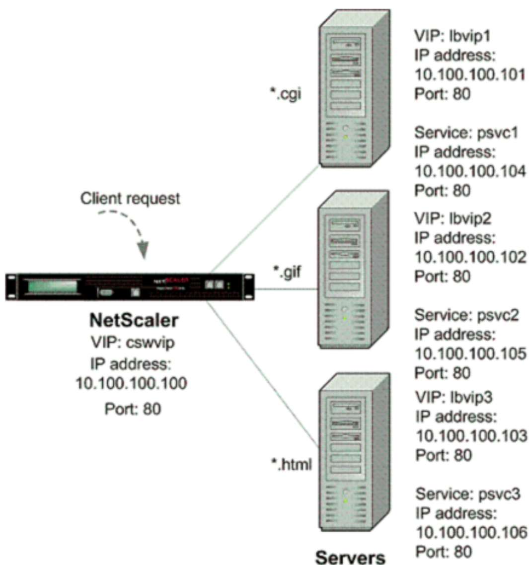
Figure 3. SureConnect Configuration - Example 5
