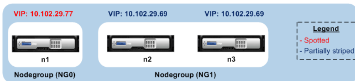
Figure 1. Citrix ADC cluster with nodegroups configured for spotted and partial-striped configurations
