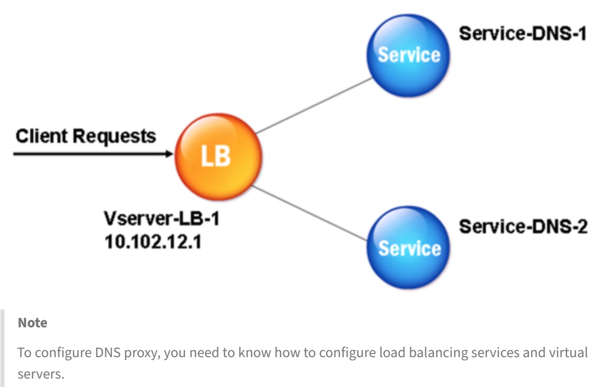
Figure 2. DNS Proxy Entity Model
