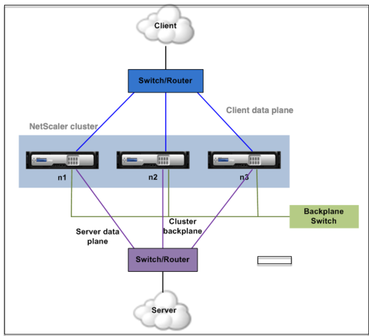
Figure 3. Cluster communication interfaces - L3 cluster
