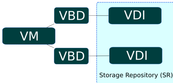
Figure 3.2. A VM object with 2 associated VDIs
